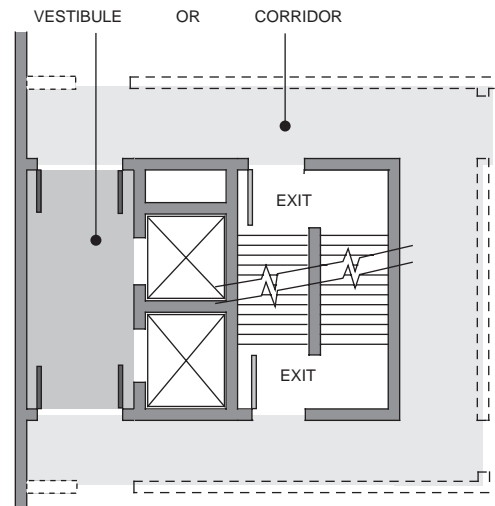
FIGURE 3.8.61. – Protected Elevator
