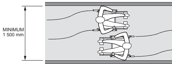
FIGURE 3.8.16. – Corridor Width
