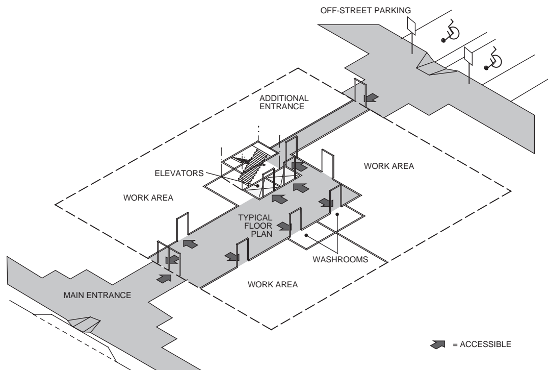
FIGURE 3.8.2. – Specific Requirements
