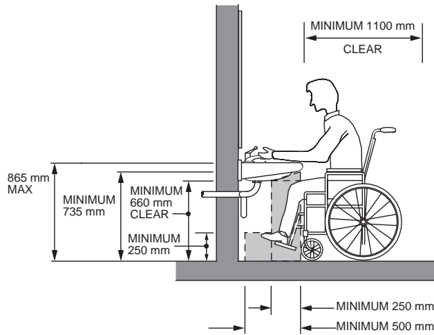
FIGURE 3.8.49. – Clearance Under Wash Basin
