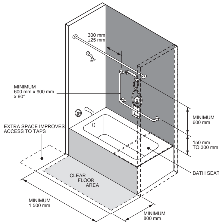
FIGURE 3.8.53. – Bath
