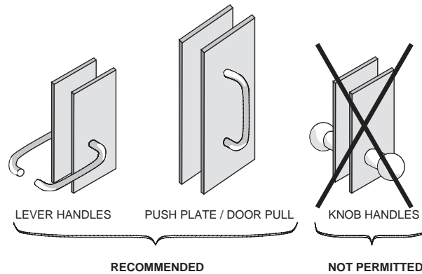
FIGURE 3.8.24. – Door Hardware
