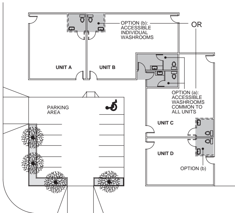
FIGURE 3.8.4. – Washrooms in Group D and E Occupancies
