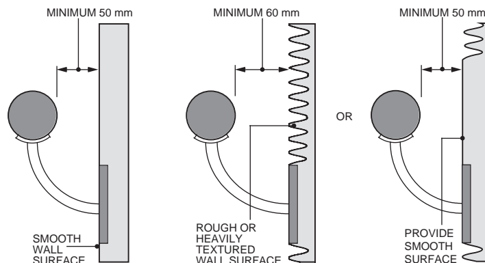
FIGURE 3.8.38. – Handrail Clearances
