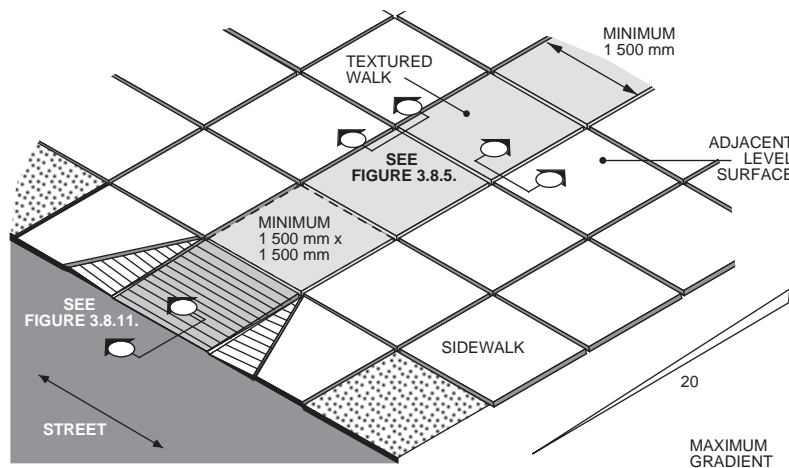
FIGURE 3.8.6. – Walks
