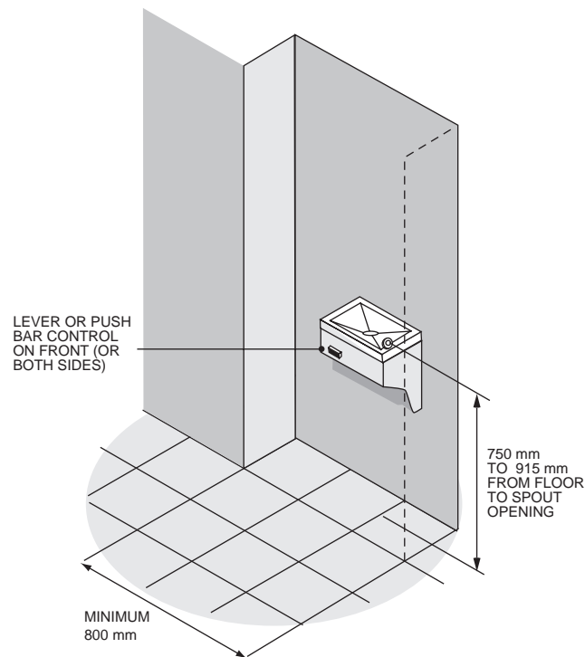
FIGURE 3.8.59. – Drinking Fountain
