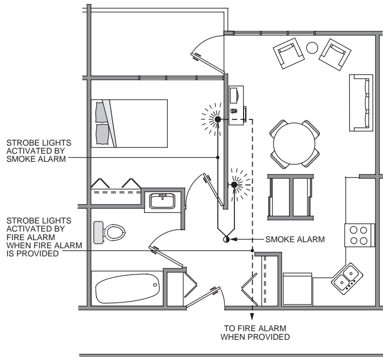
FIGURE 3.8.40. – Strobe Lights
