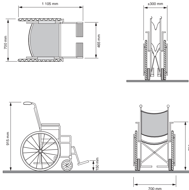
FIGURE A.3.8.1.
