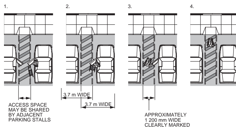
FIGURE 3.8.14. – Parking Stalls
