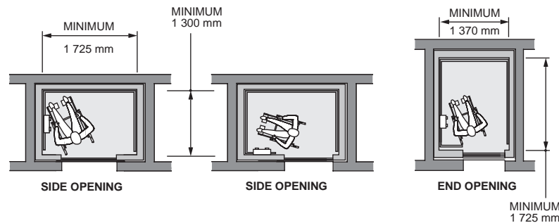
FIGURE 3.8.31. – Elevator Car Size and Operating Panel Location
