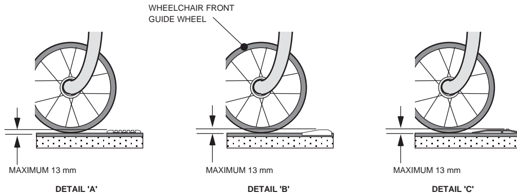
FIGURE 3.8.26. – Thresholds
