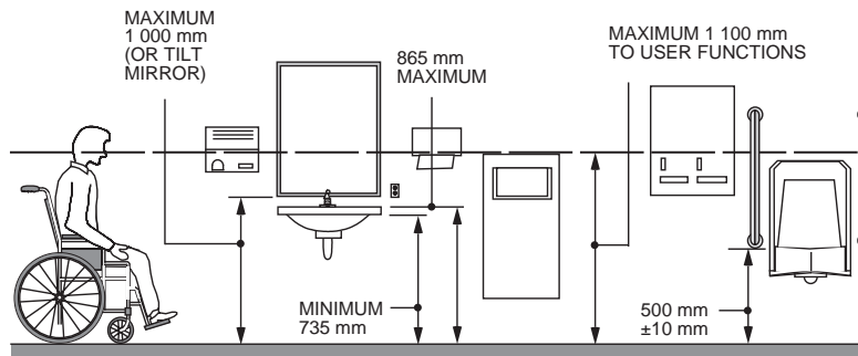
FIGURE 3.8.51. – Washroom Accessories
