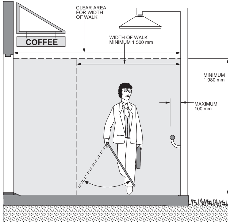
FIGURE 3.8.7. – Exterior Paths of Travel
