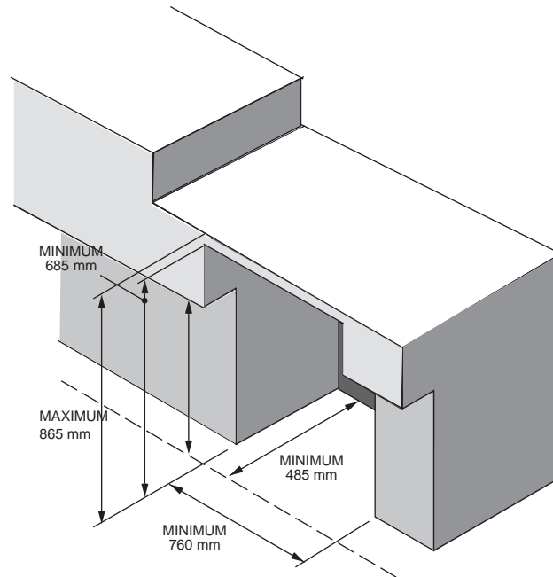
FIGURE 3.8.60. – Counter
