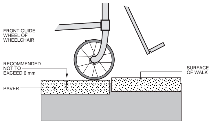
FIGURE 3.8.5. – Joints in Walks
