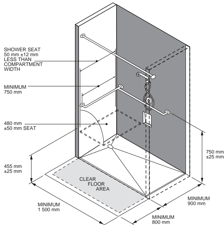
FIGURE 3.8.54. – Shower Compartment
